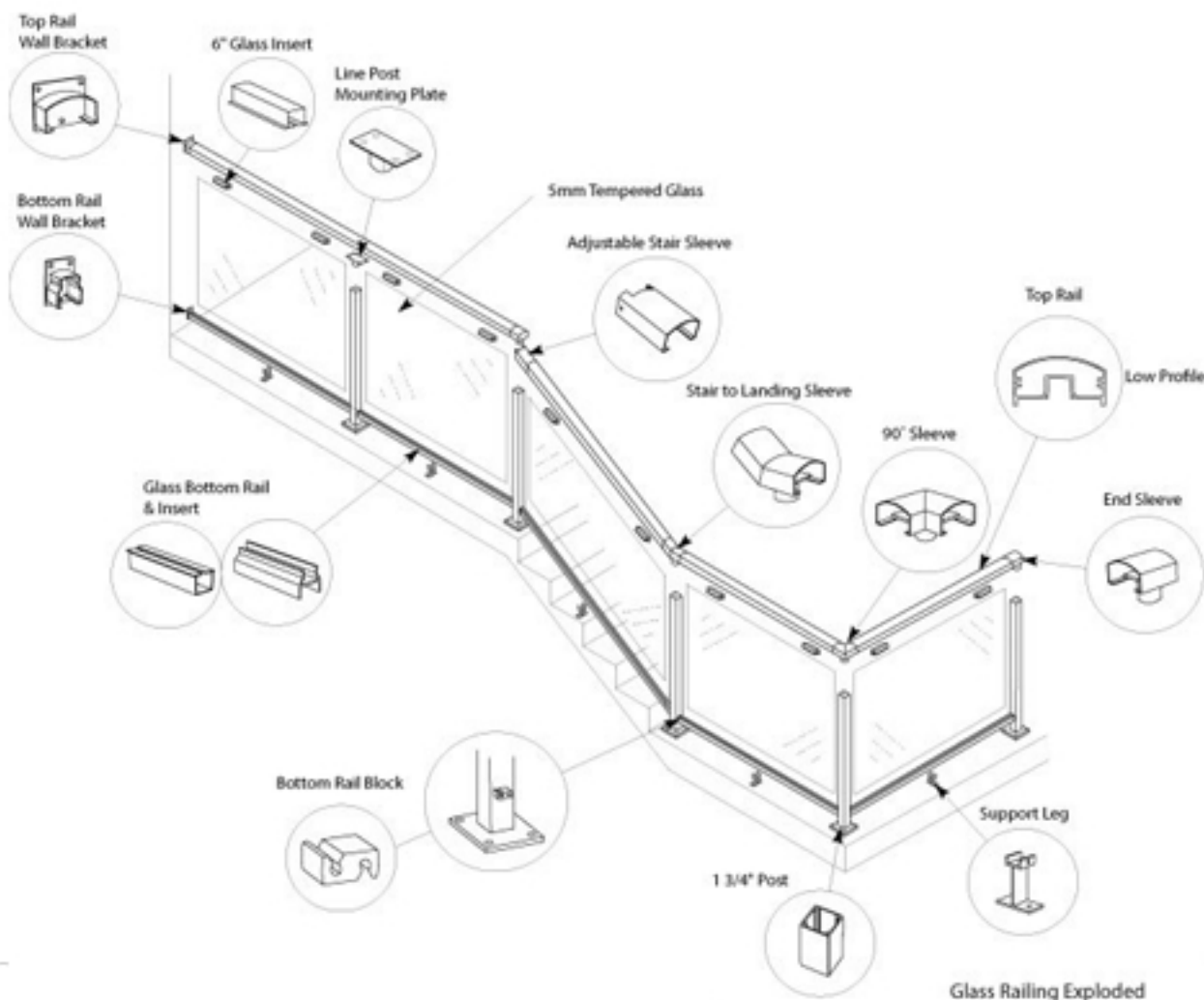
Glass Railing Exploded
